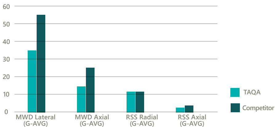
Vibration Comparison 6 1/4" Vertical, Curve, Lateral – British Columbia, Canada
