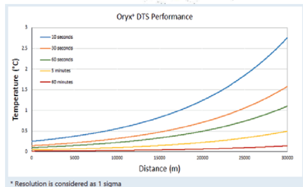
The graph illustrates the temperature resolution* of each Oryx+ DTS with sensing range and measurement time
